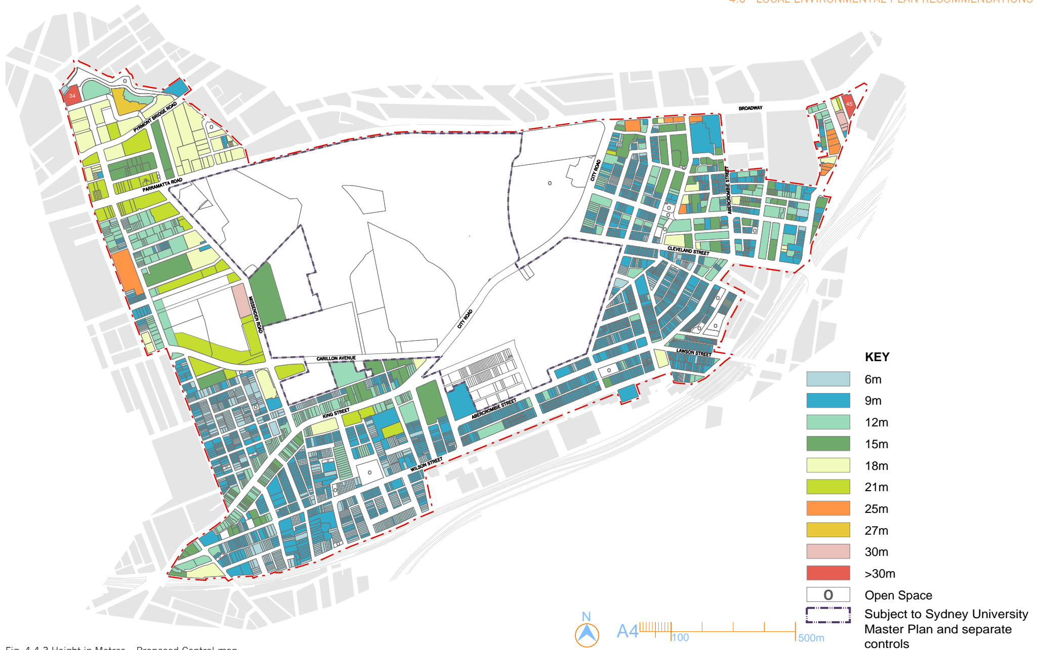
Fig. 4.4.3 Height in Metres – Proposed Control map (shown using the standard instrument definition of building height)
