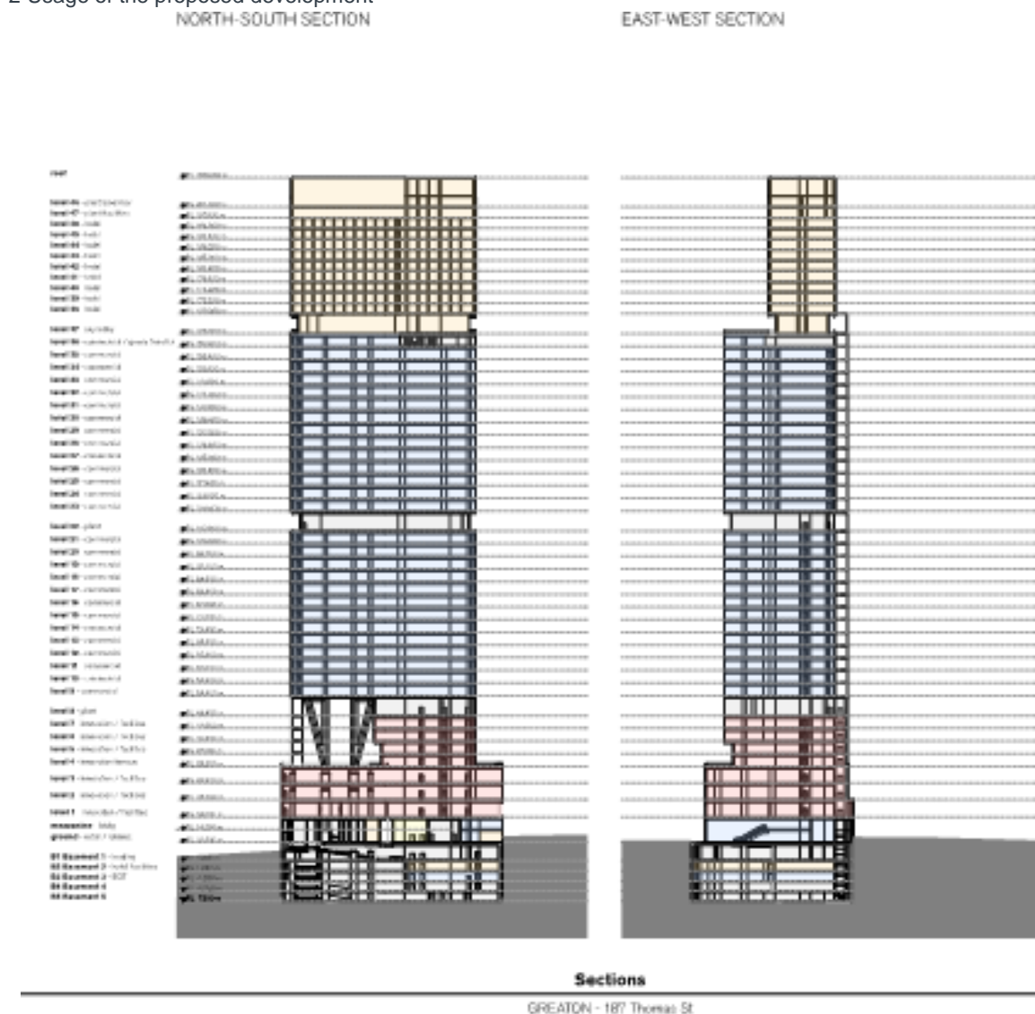
Figure 1 - 187 Thomas Street Section Drawing
