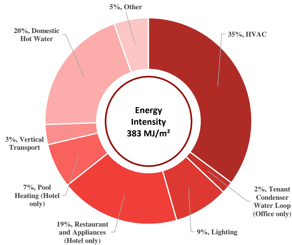
Figure 3 Energy Intensity Breakdown before Renewable Energy
