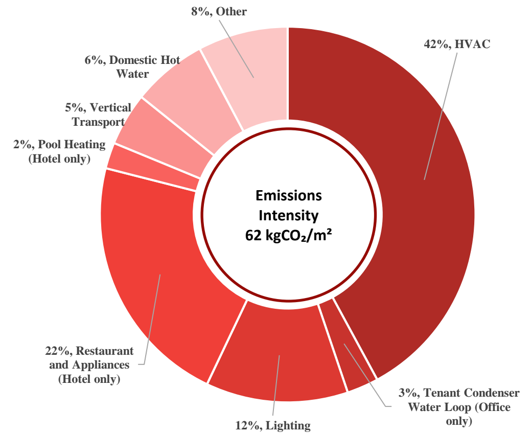
Figure 4 Emissions Intensity Breakdown before Renewable Energy
