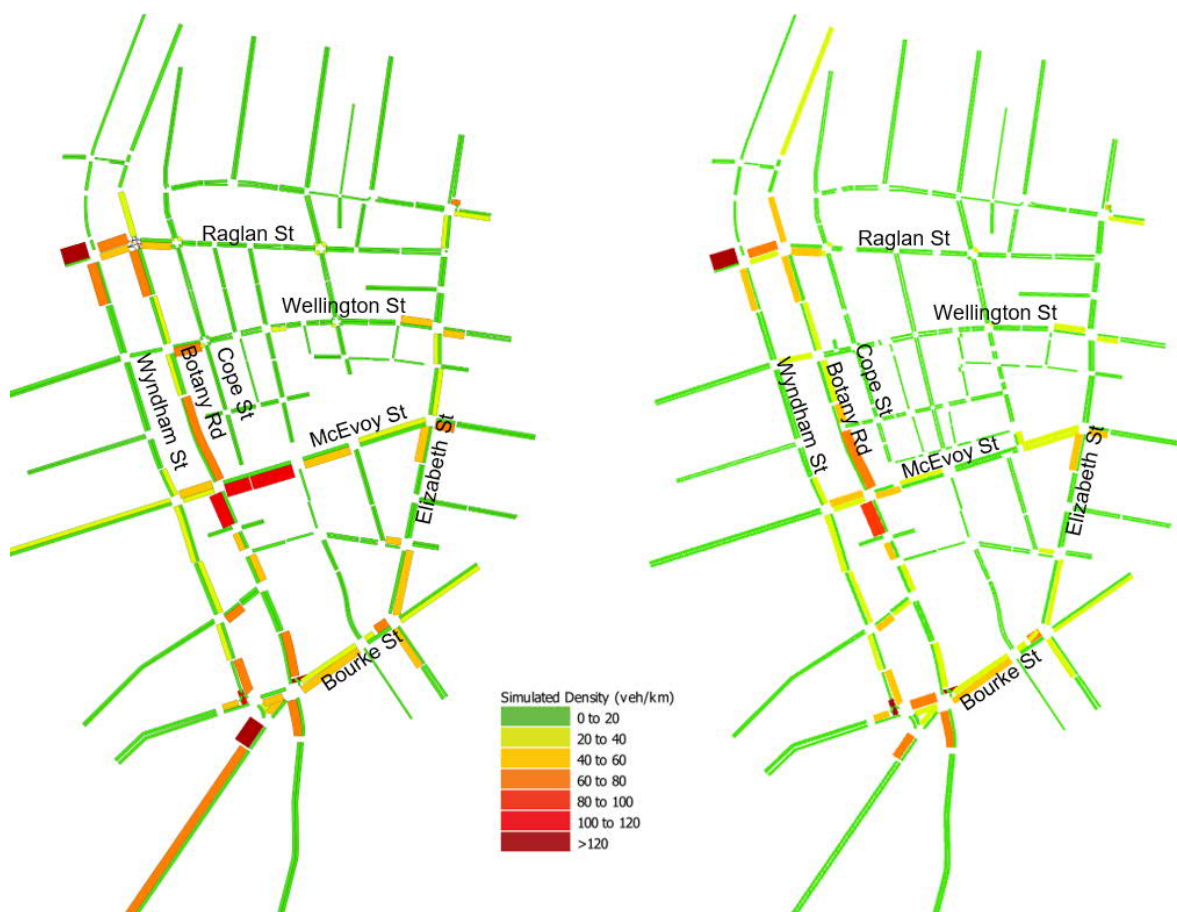
Figure 6.12: Simulated density 2036 morning peak: do minimum (left) and with development (right)
