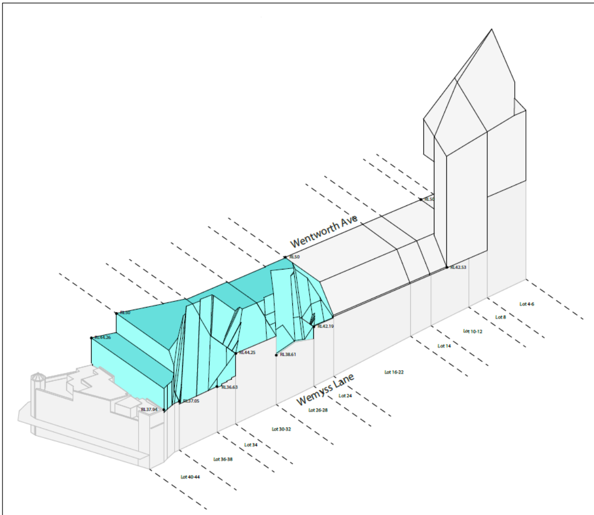
Figure 6xxx: 24-44 Wentworth Avenue: Maximum planning envelope – axonometric view 2
