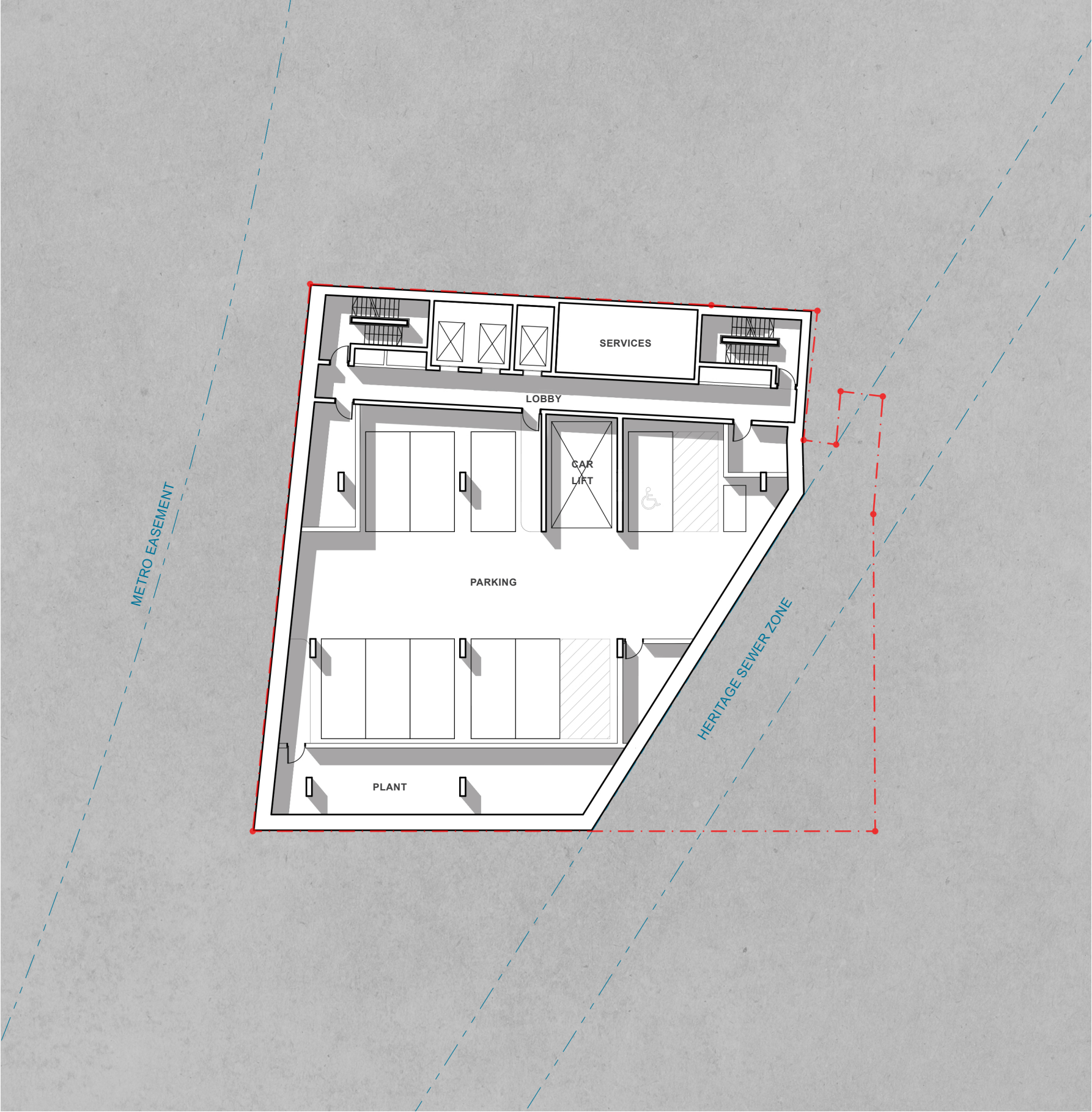
BASEMENT 2-3 PLAN
