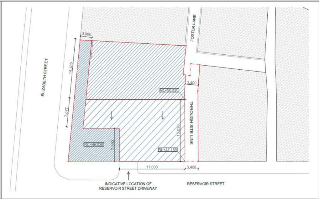
Figure 6.1.## 232-240 Elizabeth Street, Surry Hills - Maximum building envelope plan
