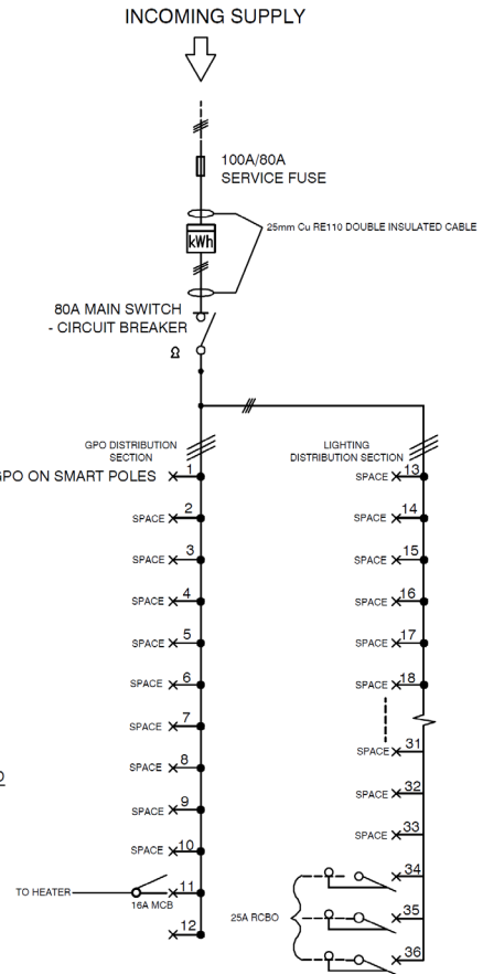
SINGLE LINE DIAGRAM
