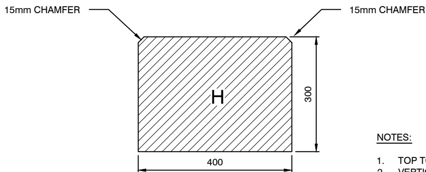
MEDIAN KERB (MK2)
