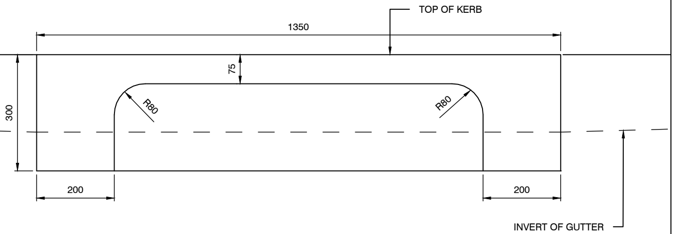
ELEVATION 1:10
