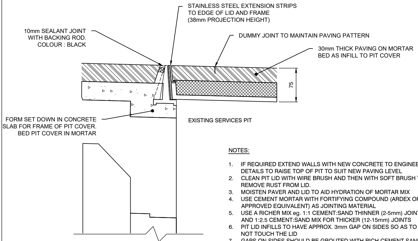
SECTION 1:5
