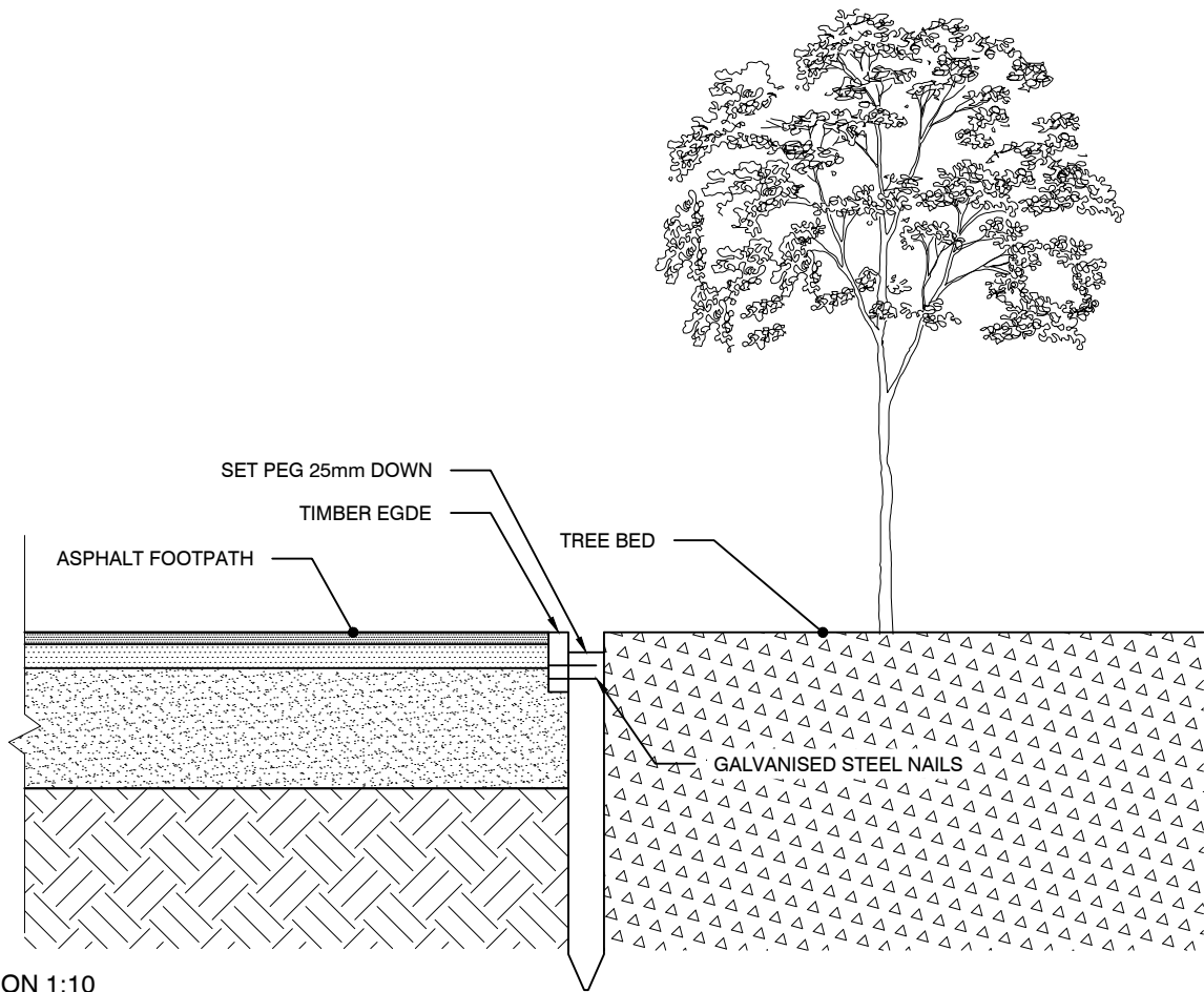
SECTION 1:10
