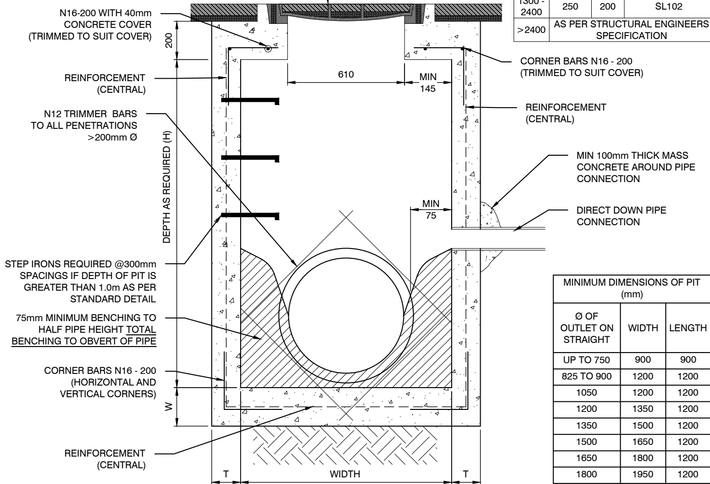
SECTION 1:20
