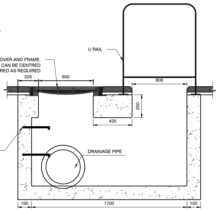
SECTION B-B 1:25
