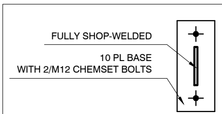
U RAIL BASE PLATE DETAIL 1:10
