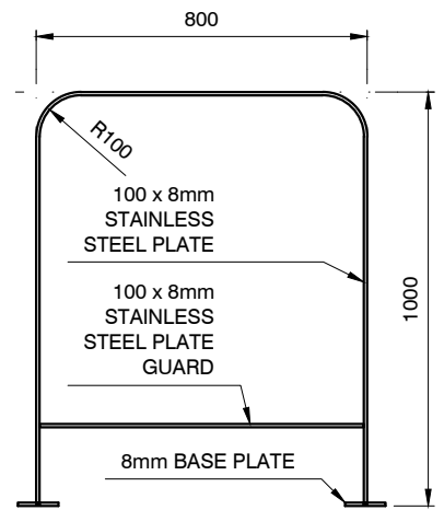
U RAIL DETAIL 1:20
