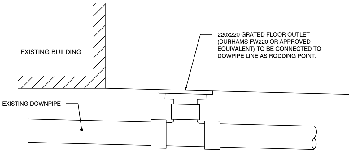
DETAIL 1:10
