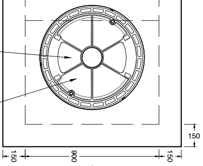
MANHOLE COVER AND FRAME. NOTE: PIT LID CAN BE CENTRED OR OFF-CENTRED AS REQUIRED
