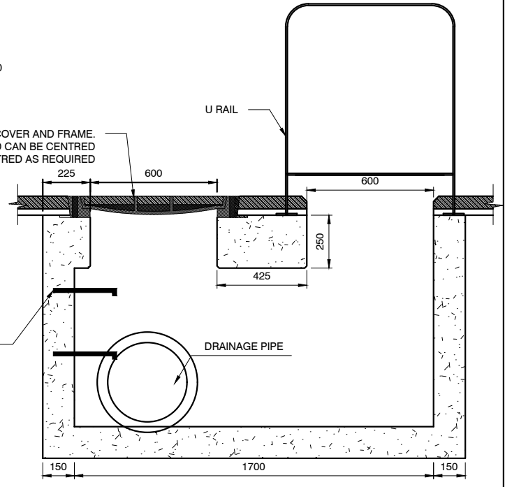
SECTION B-B 1:25
