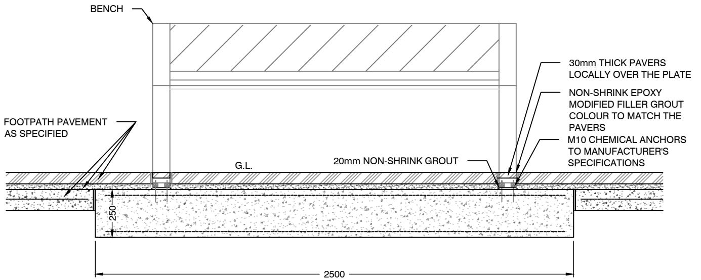
SECTION 1:20
